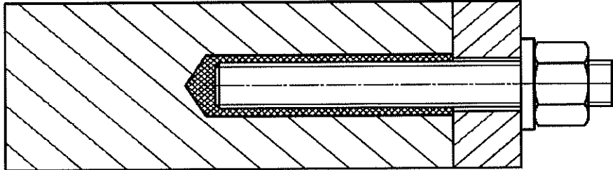
Standard threaded rod with flat tip end
