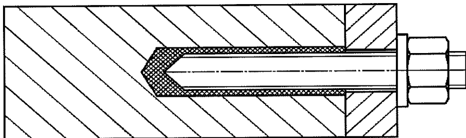
Standard threaded rod with two sides 45° chamfer
