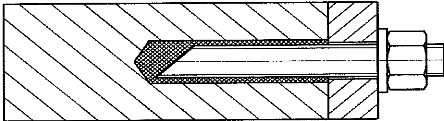
Standard threaded rod with one side 45° chamfer
