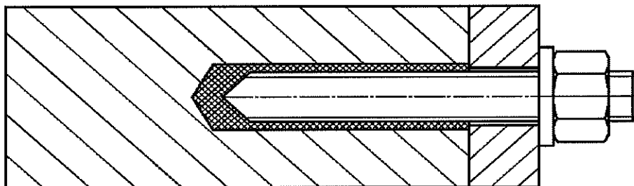
Standard threaded rod with two sides 45° chamfer
