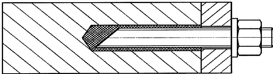
Standard threaded rod with one side 45° chamfer
